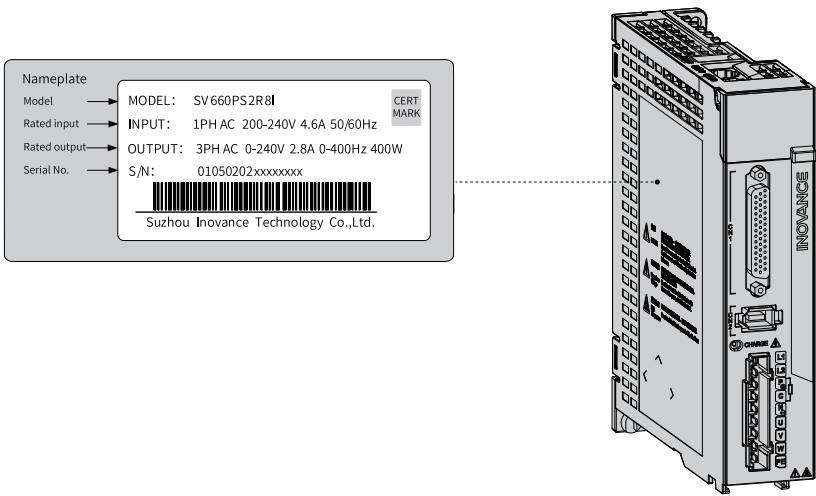
Figure 2-1 Nameplate
