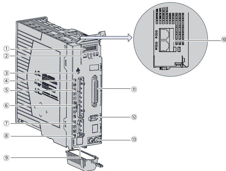
Figure 2-5 Components of servo drives in size C and size D (size C: SV660PT3R5I and SV660PT5R4I; size D: SV660PT8R4I and SV660PT012I)
