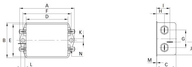
Figure 4-4 Dimensions of FN 2090 series filters (unit: mm)
