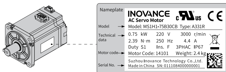
Figure 3-1 Description of the model and nameplate
