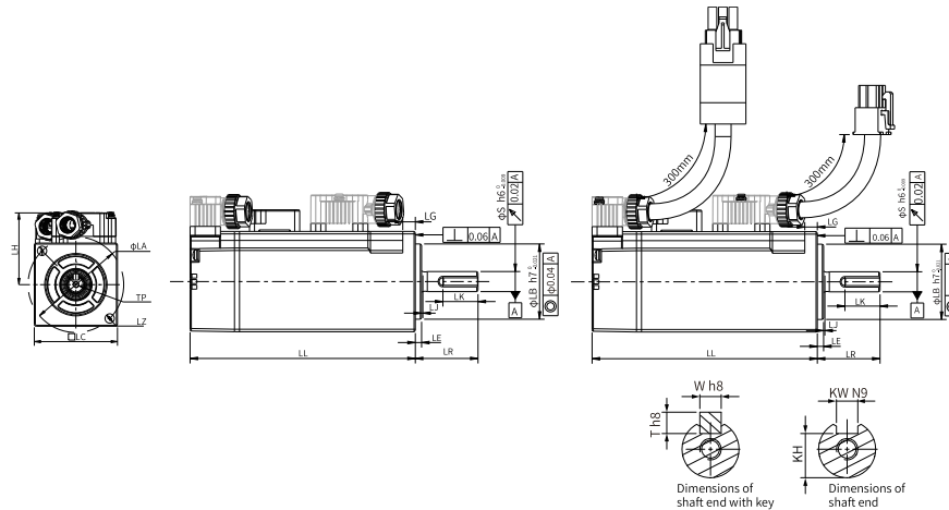
Figure 4-6 MS1H4-10B30CB-A6/S631R and MS1H4-10B30CB-A6/S634R
