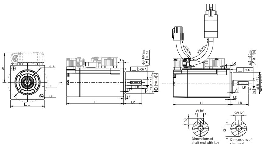
Figure 4-2 MS1H4-05B30CB-A6/S631R and MS1H4-05B30CB-A6/S634R
