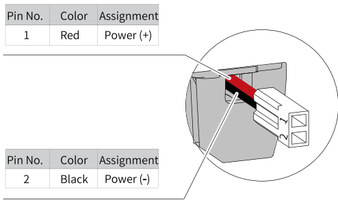
Figure 5-4 Lead wire color of the battery box
