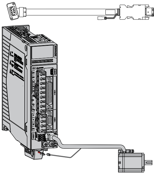
Figure 5-3 Wiring example of absolute encoder signals [1]
