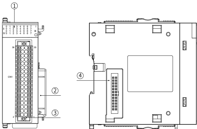
Figure 2 Diagram of digital input module interface
